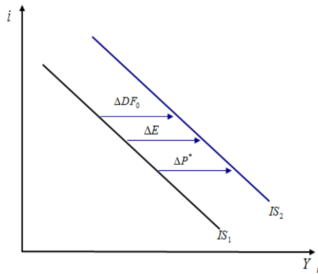
Figura 1: La Curva IS
